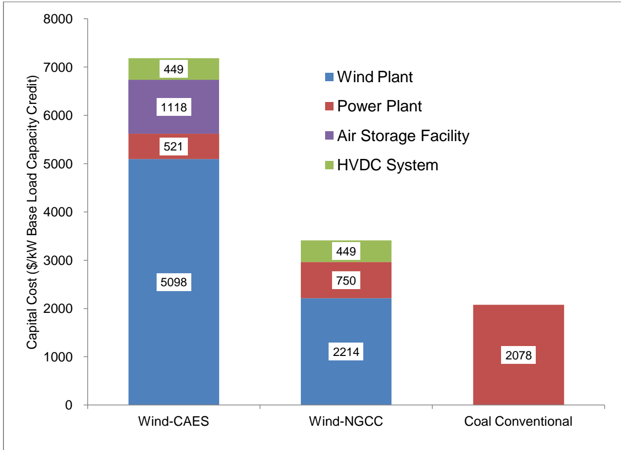
Figure 8. Capital cost components of the Wind-NGCC, Wind-CAES, and Coal models. Compressor cost for the Wind-CAES model is included in the air storage facility since the compressors are assumed separate from the CAES CT plant's turbotrain.
