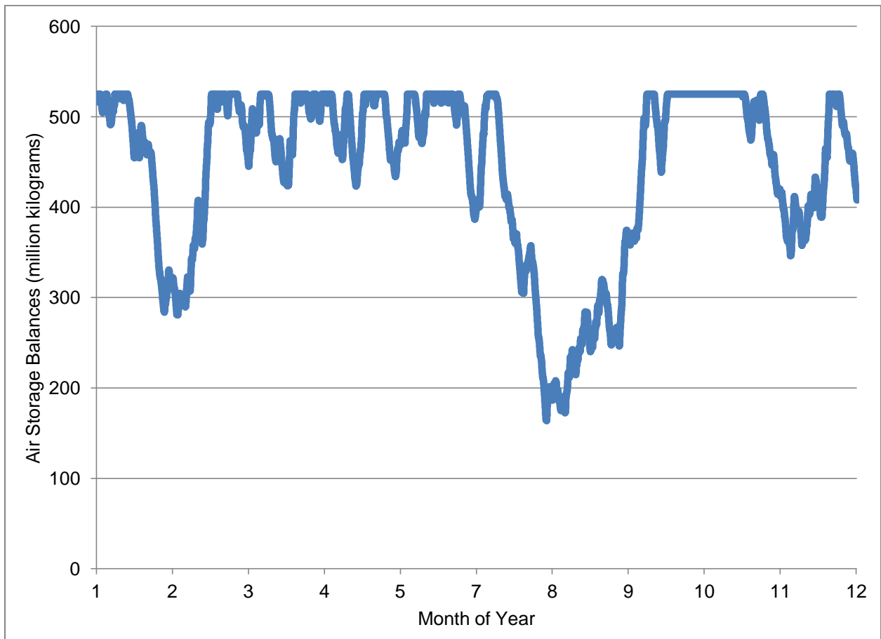
Figure 6. Air storage balance (million kg) for Wind-CAES model with 290 hours of air storage capacity. Notice that there is a 30% air storage margin, 160 million kg, in late summer for years with lowest quality wind conditions.
