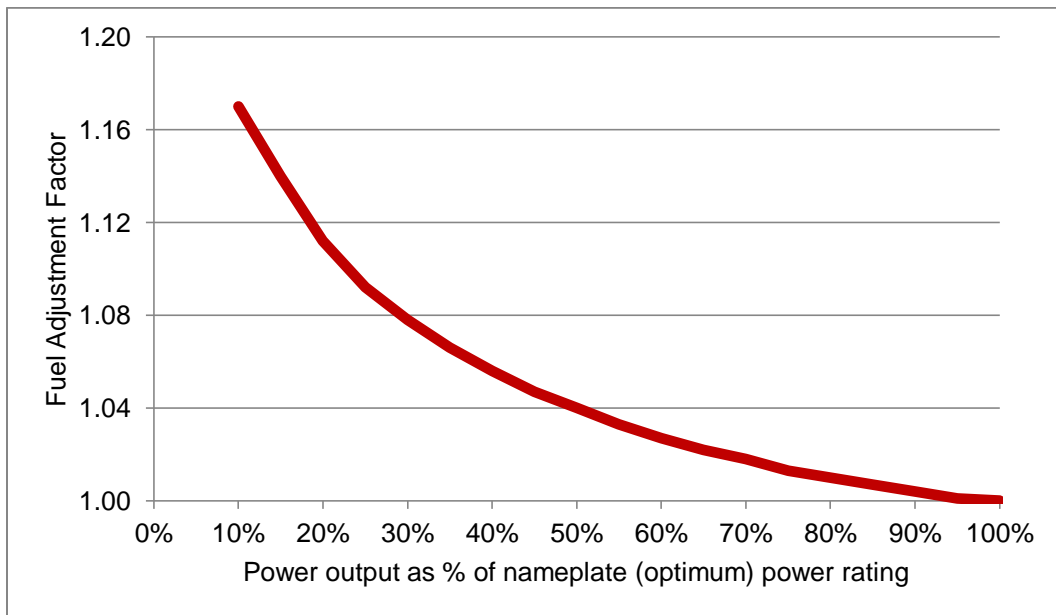
Figure 4. Power plant heat rate adjustment factors, which are derived from EPRI and Dresser-Rand estimates [26, 27].
