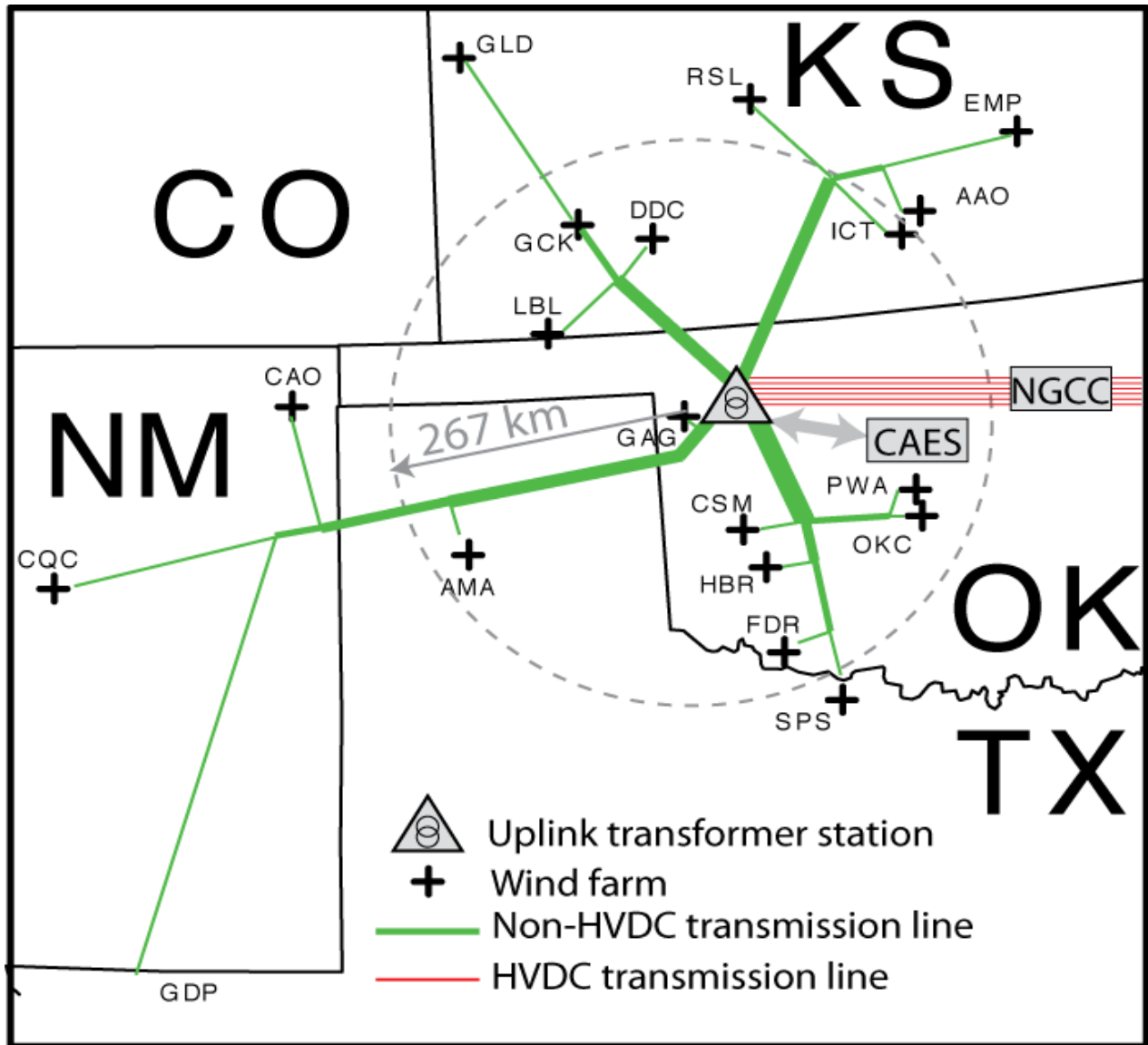
Figure 3. Schematic of the model wind farm, CAES, and HVDC uplink system. The + marks are the locations of the 19 interconnected wind plants used in this study. The CAES plant and the HVDC transformer station are located in close proximity. The NGCC plant, alternatively to CAES, would be located downwind of the HVDC uplink station.
