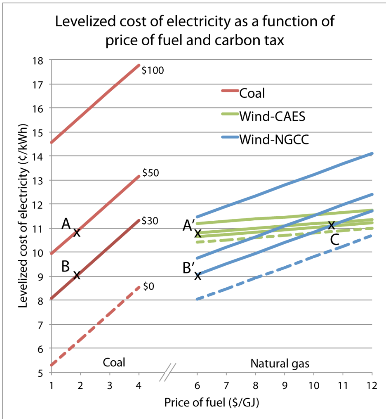
Figure 9. Levelized cost of electricity (¢/kWh) from Coal, Wind-NGCC, and Wind-CAES as a function of price of fuel ($/GJ, either coal or natural gas) for various carbon taxes (none, $30, $50, and $100 per metric ton of CO 2 ). Pair A-A' indicates cost parity between Coal and Wind-CAES (at ~11 ¢/kWh with coal at ~$2/GJ, natural gas at ~$6/GJ, and a carbon tax of $50/ton-CO 2 ), B-B' between Coal and Wind-NGCC (~9 ¢/kWh with carbon tax of $30/ton-CO 2 ), and point C between Wind-NGCC and Wind CAES (~11 ¢/kWh with natural gas at ~$10.5/GJ and carbon tax of $30/ton-CO 2 ).
