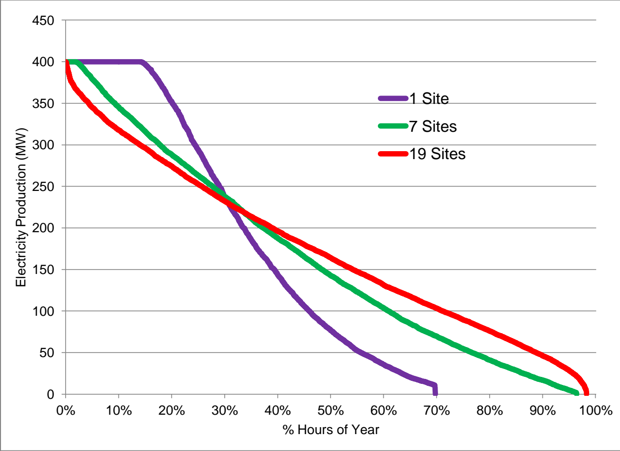
Figure 2. The effect of interconnecting geographically dispersed wind plants on aggregate power supply.
