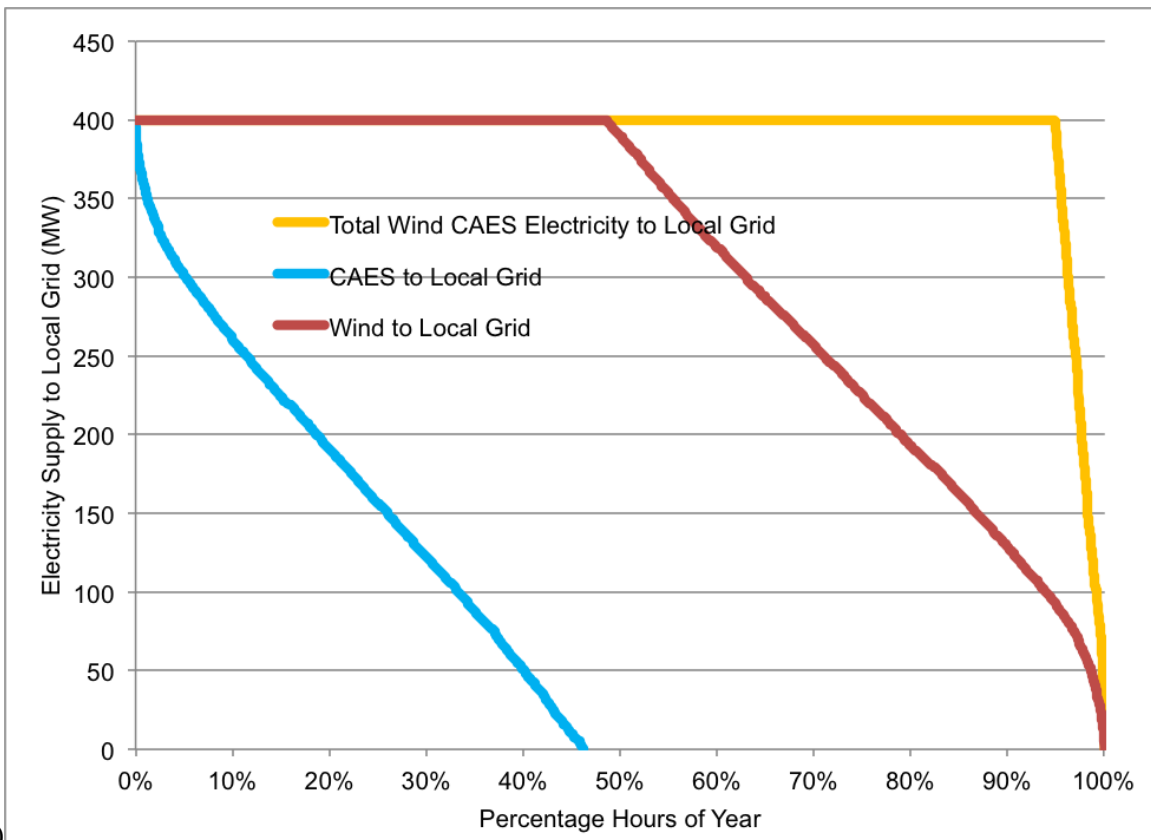
Figure 5. Wind-NGCC (a) and Wind-CAES (b) power duration curves.
